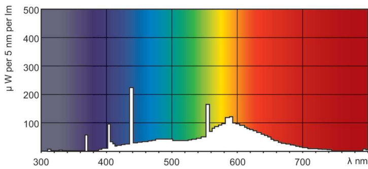
Spectral Power Distribution Colour - F15T8/CW 25PK
